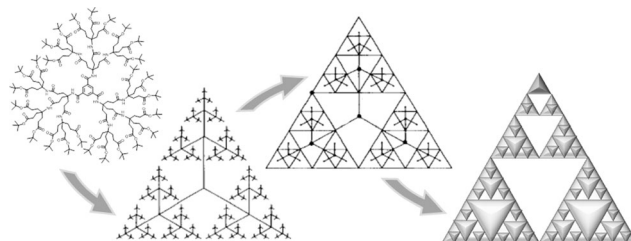
Figure 1. Conceptual progression of a 1→3 dendritic branching pattern and its geometric relationship to the classical Sierpiński triangle. [10]
